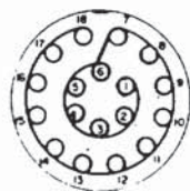
PI-C WIRING VIEW
